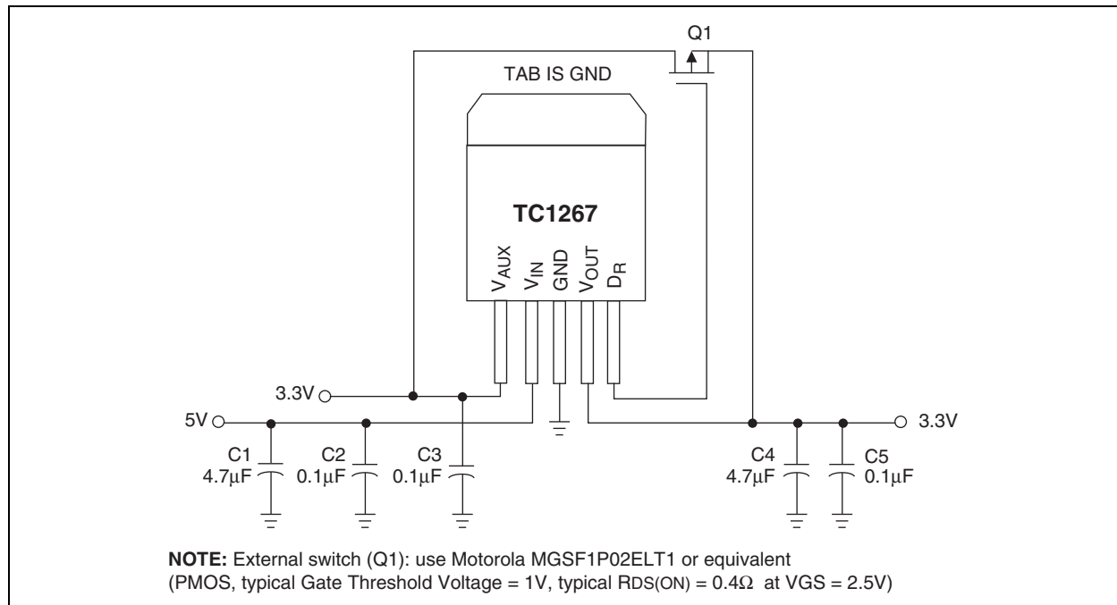
FIGURE 3-1: APPLICATION CIRCUIT
