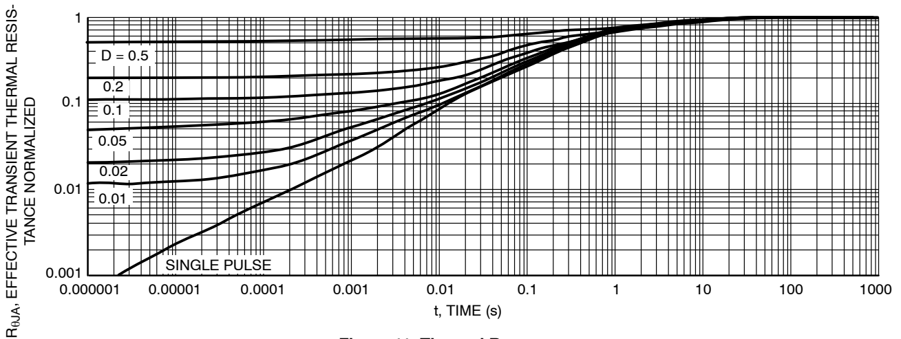
Figure 11. Thermal Response
