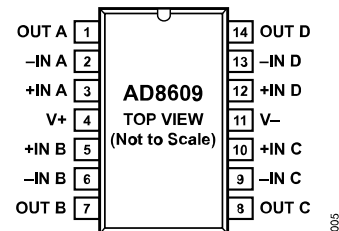
Figure 5. 14-Lead SOIC (R Suffix)
