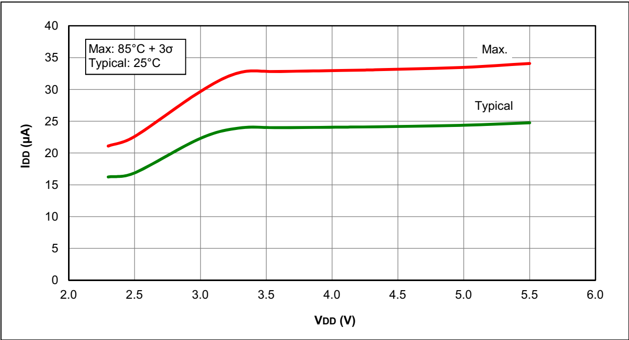
FIGURE 26-8: I_{DD} , EXTERNAL CLOCK (ECL), LOW-POWER MODE, F_{osc} = 32\text{ kHz} , PIC16F1526/7 ONLY
