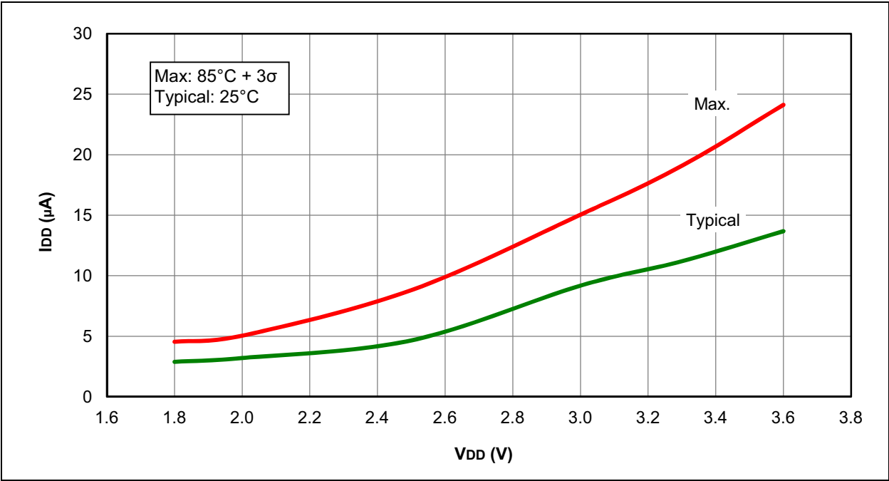
FIGURE 26-7: I_{DD} , EXTERNAL CLOCK (ECL), LOW-POWER MODE, F_{osc} = 32\text{ kHz} , PIC16LF1526 ONLY
