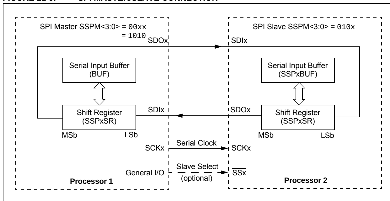
FIGURE 21-5: SPI MASTER/S�AVE CONNECTION
