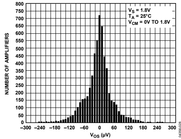
Figure 28. V_{OS} Distribution
