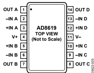
Figure 4. 14-Lead TSSOP and 14-Lead SOIC
