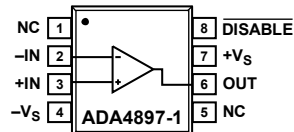
Figure 6. 8-Lead SOIC Pin Configuration
