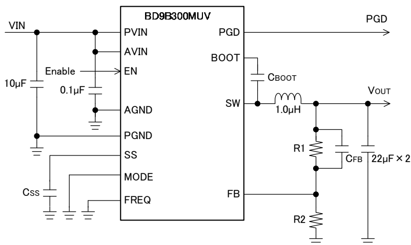
Figure 1. Application Circuit
