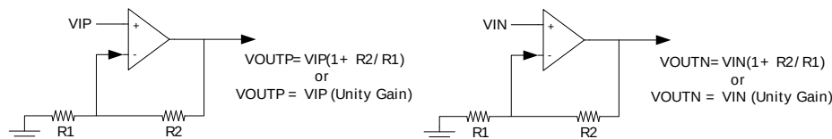
Figure 26.11. Dual Buffer ADC Driver Overview
