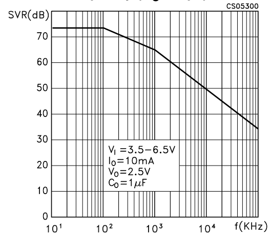
Figure 12. Supply voltage rejection vs. frequency ( C_o = 1 \mu\text{F} )
