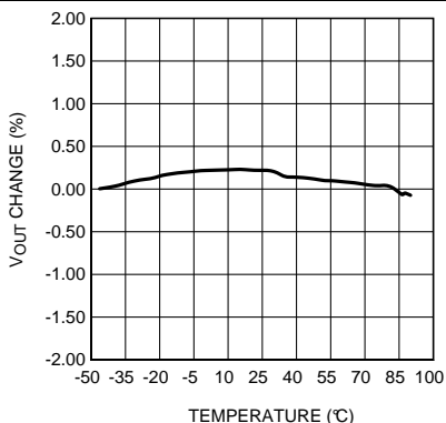
V IN = 3.6 V V OUT = 2.6 V 100-mA Load Figure 1. Output Voltage Change vs Temperature (LDO1)
