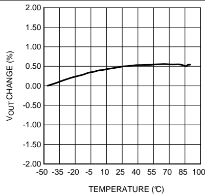
V IN = 3.6 V V OUT = 2.6 V 100-mA Load Figure 2. Output Voltage Change vs Temperature (LDO2)
