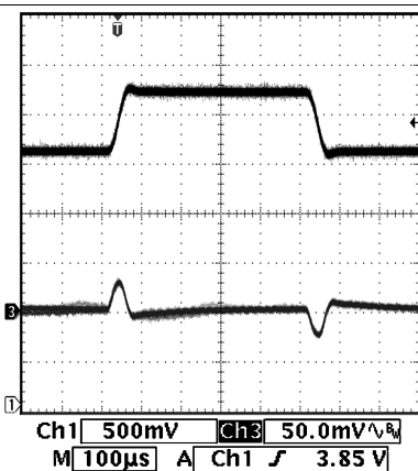
V IN = 3.6 to 4.2 V V OUT = 2.6 V 300-mA Load Figure 5. Line Transient (LDO1)
