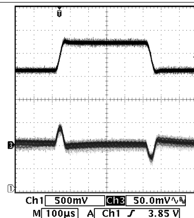
V IN = 3.6 to 4.2 V V OUT = 3.3 V 300-mA Load Figure 6. Line Transient (LDO2)
