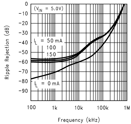
Ripple Rejection ( V_{IN} = 5.0V )
