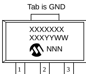
3-Lead SOT-223
