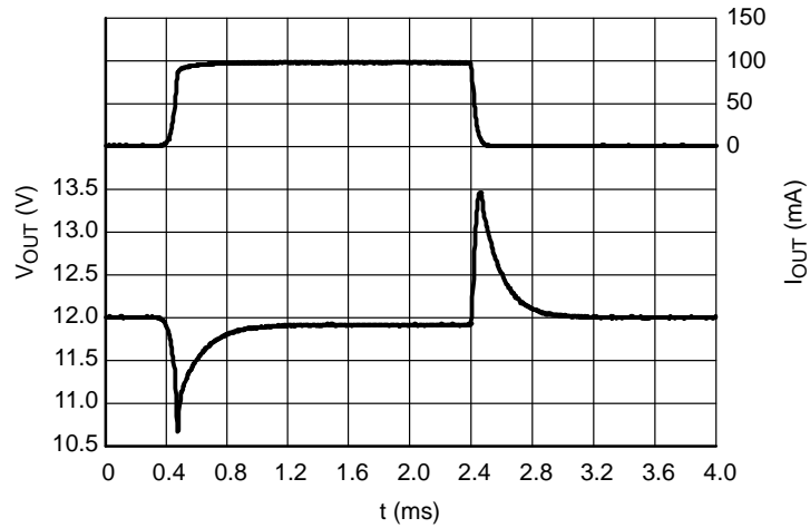
Figure 40. Load Transients, 12.0 V Version, I_{OUT} = 1 - 100 mA, t_R = t_F = 50 \mu s, V_{IN} = 14.0 V
