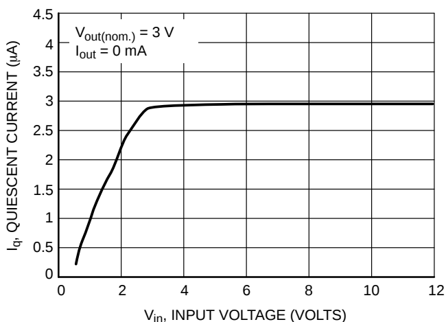
Figure 6. Quiescent Current versus Input Voltage
