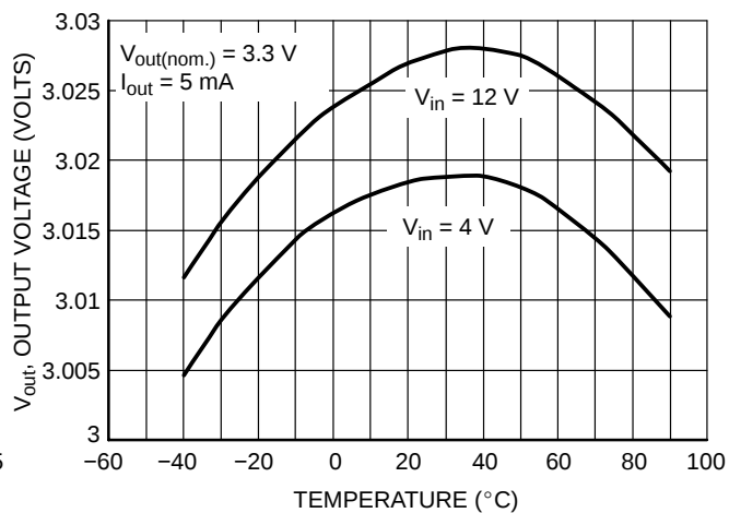
Figure 4. Output Voltage versus Temperature
