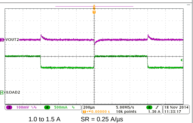
Figure 53. BUCK2, Load Transient
