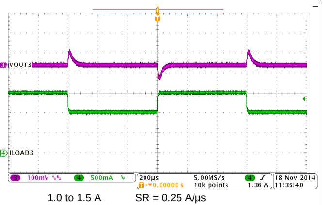
Figure 55. BUCK3, Load Transient
