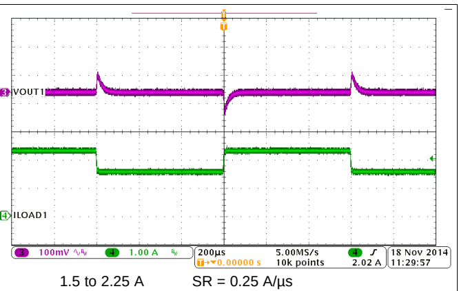
Figure 51. BUCK1, Load Transient
