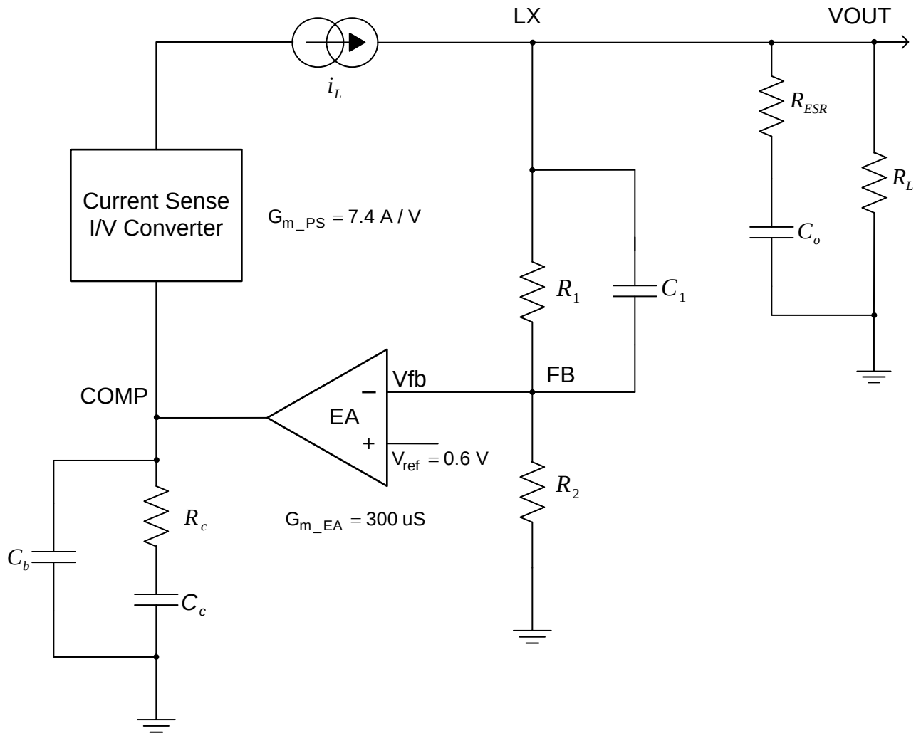
Figure 43. DC/DC Loop Compensation
