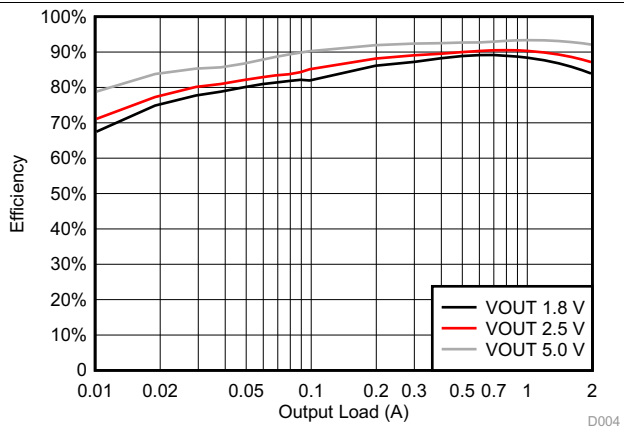
Figure 1. BUCK1 Efficiency
