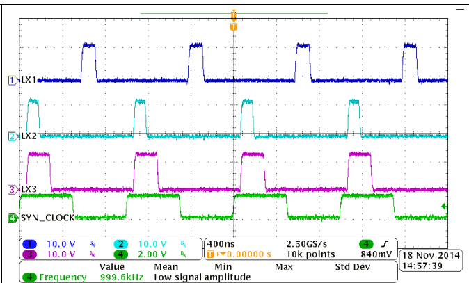
Figure 63. Synchronization With External Clock
