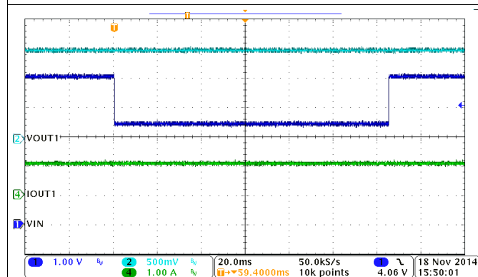
Figure 62. 180° Out-of-Phase
