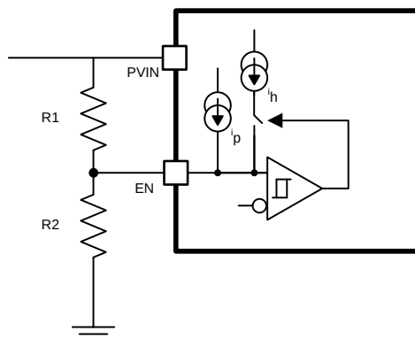
Figure 24. Adjustable PVIN UVLO, VIN &gt; 4 V
