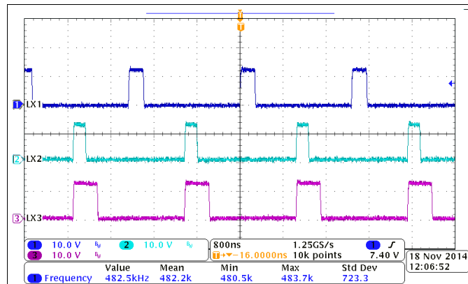
Figure 62. 180° Out-of-Phase
