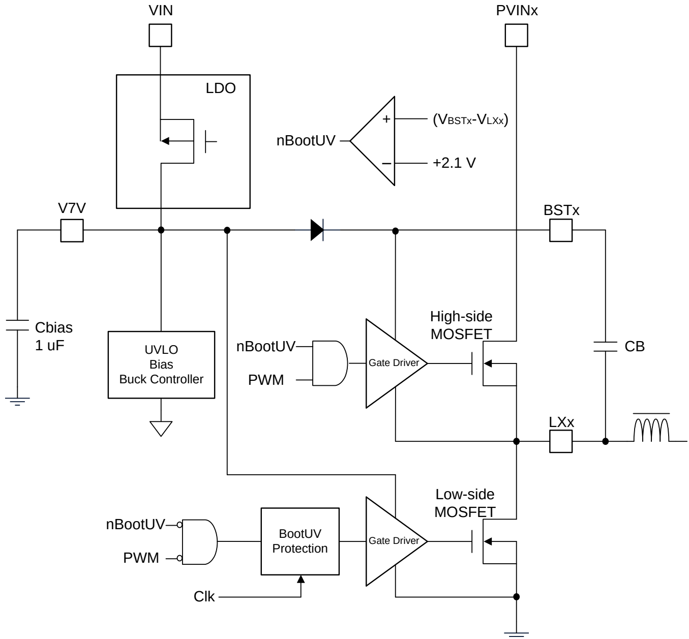
Figure 29. V7V Linear Dropout Regulator and Bootstrap Voltage Diagram
