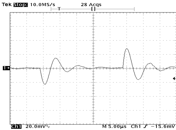
FIGURE 24. LINE TRANSIENT RESPONSE, 0.001µF LOAD CAPACITANCE
