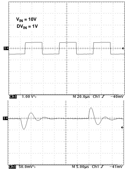
FIGURE 52. LINE TRANSIENT RESPONSE, 0.001µF LOAD CAPACITANCE
