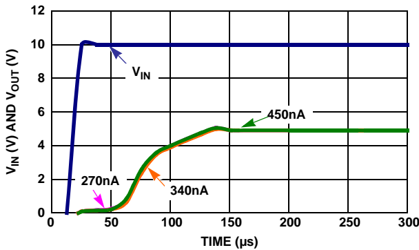
FIGURE 53. TURN-ON TIME
