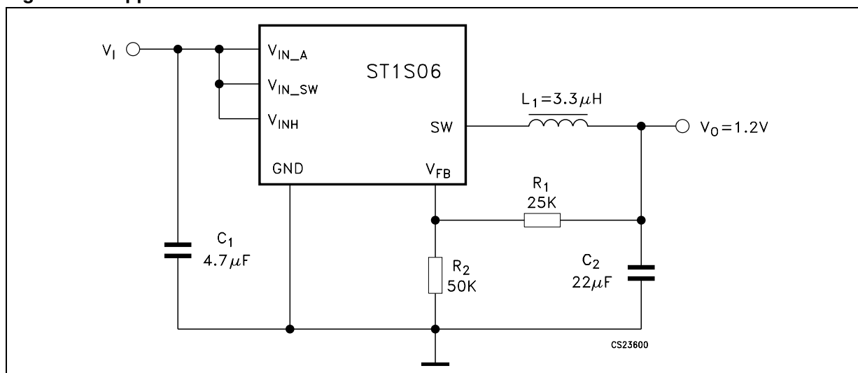
Figure 24. Application circuit
