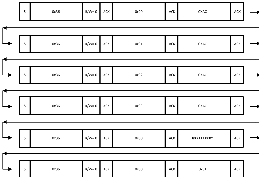
*Only bits <5:3> are necessary in this byte the rest are don't cares. Bits <5:3> = '111' are necessary to latch the pattern generator data bits into the internal shift register.
