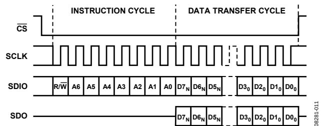
Figure 39. Serial Port Interface Timing, MSB First
