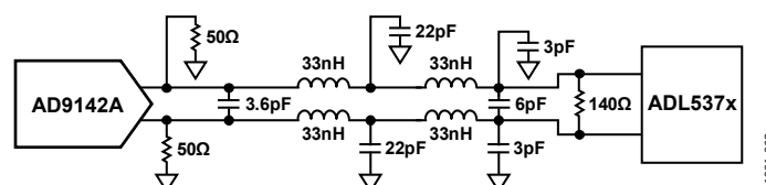
Figure 61. DAC Modulator Interface with Fifth-Order, Low-Pass Filter
