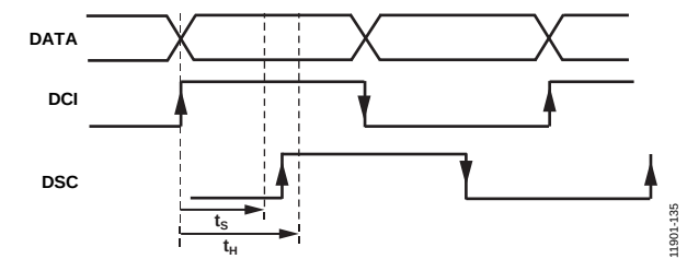
Figure 35. LVDS Data Port Setup and Hold Times
