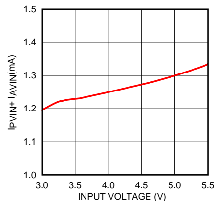
Figure 6. Non-Switching I_{QTOTAL} vs V_{IN}
