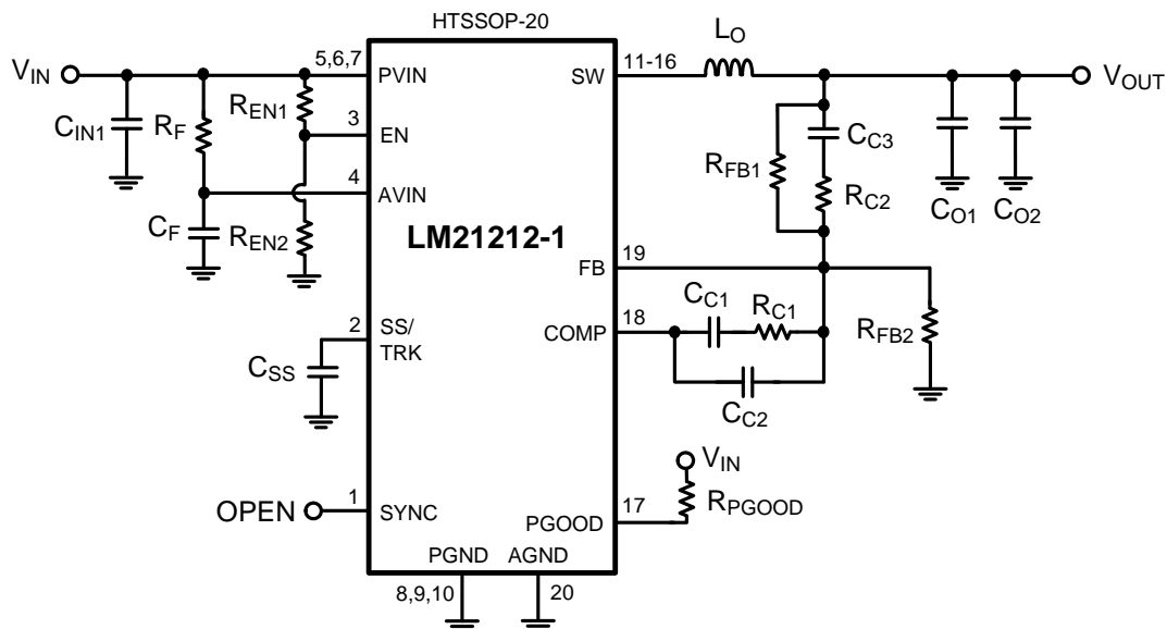
Figure 39. Typical Application Schematic 2
