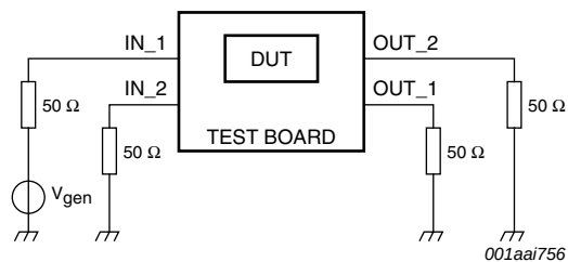
Fig 6. Crosstalk measurement configuration
