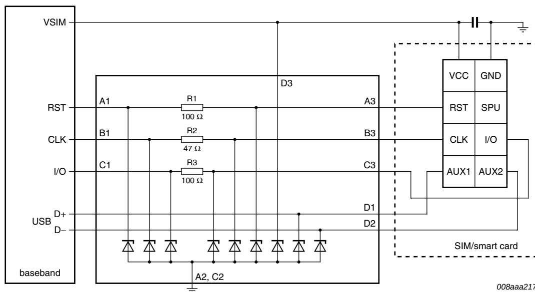
Fig 3. Typical application diagram
