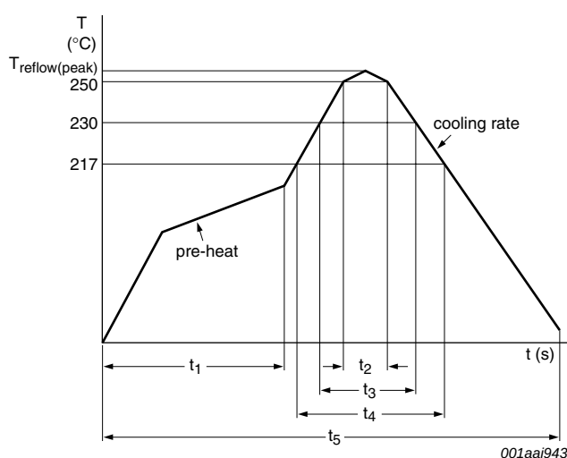
Fig 9. Pb-free solder reflow profile
