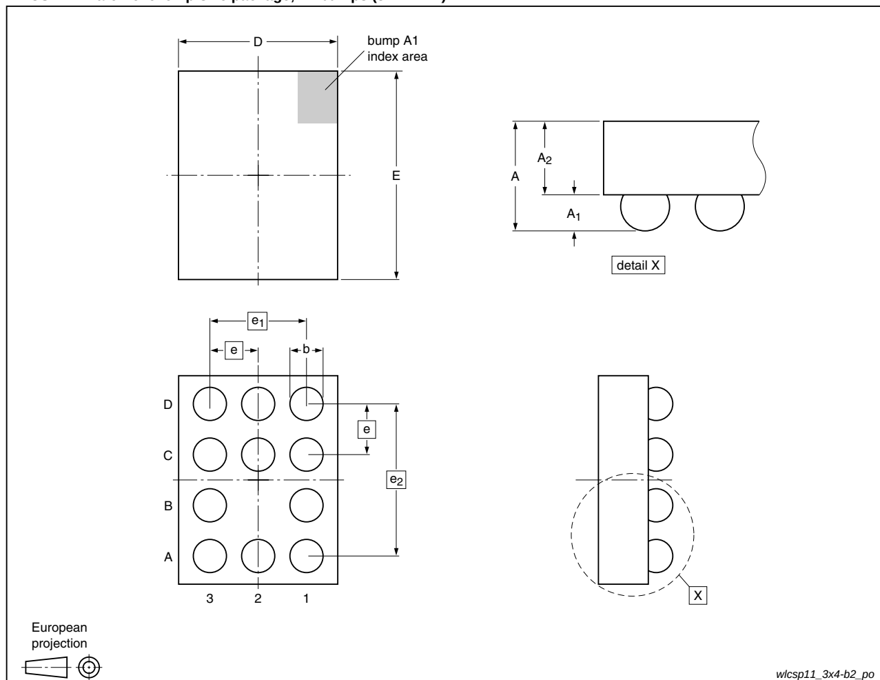
Fig 8. Package outline IP4365CX11 (WLCSP11)
