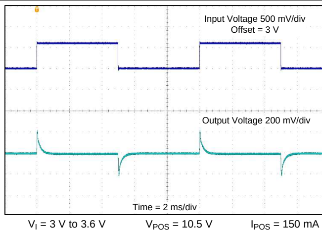
Figure 21. Boost Converter ( V_{\text{POS}} ) Line Transient Response
