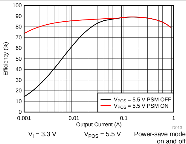
Figure 26. Boost Converter ( V_{POS} ) Efficiency vs Output Current
