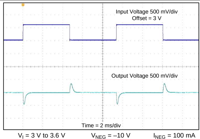
Figure 22. Inverting ( V_{\text{NEG}} ) Converter Line Transient Response
