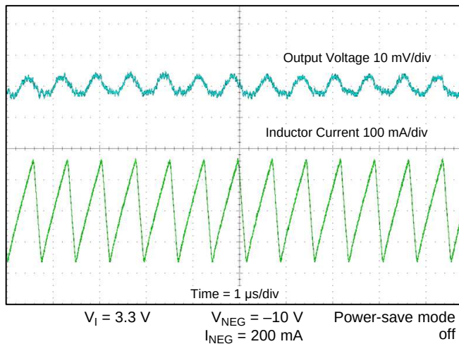
Figure 17. Inverting Converter ( V_{\text{NEG}} ) Output Ripple
