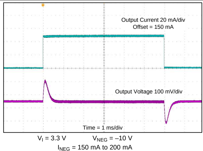
Figure 20. Inverting Converter ( V_{\text{NEG}} ) Load Transient Response
