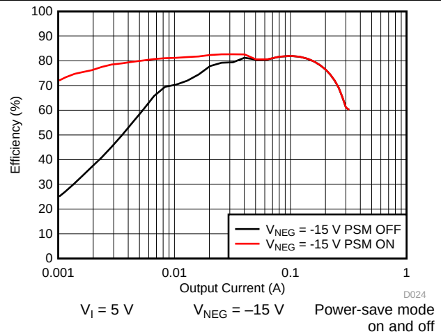
Figure 37. Inverting Converter ( V_{NEG} ) Efficiency vs Output Current
