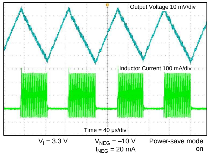
Figure 18. Inverting Converter ( V_{\text{NEG}} ) Output Ripple
