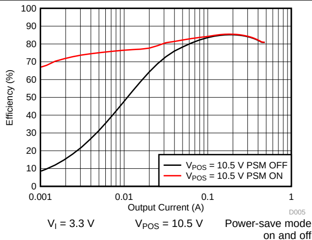
Figure 7. Boost Converter ( V_{POS} ) Efficiency vs Output Current
