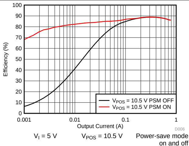
Figure 8. Boost Converter ( V_{POS} ) Efficiency vs Output Current
