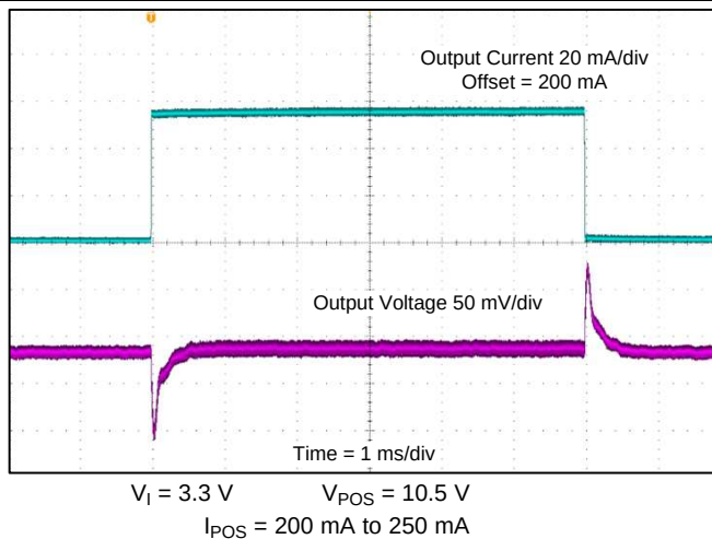
Figure 19. Boost Converter ( V_{\text{POS}} ) Load Transient Response
