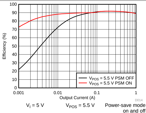
Figure 27. Boost Converter ( V_{POS} ) Efficiency vs Output Current
