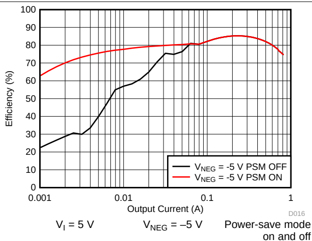
Figure 29. Inverting Converter ( V_{NEG} ) Efficiency vs Output Current
