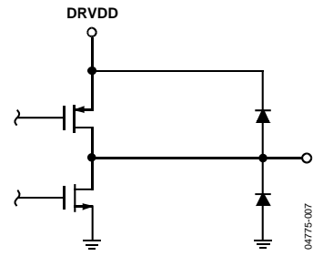
Figure 40. Digital Outputs
