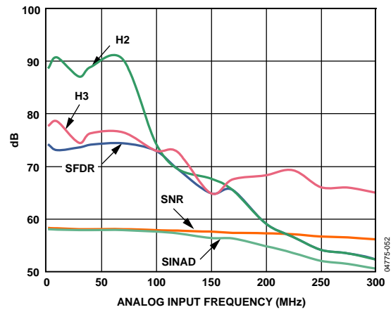
Figure 14. Analog Input Frequency Sweep, A_{IN} = -0.5 dBFS, f_s = 65 MSPS ( -65 Grade)
