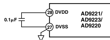
Figure 32. Digital Supply Decoupling
