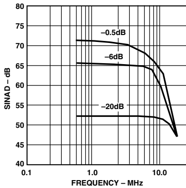
TPC 22. SINAD vs. Input Frequency (Input Span = 2.0 V p-p, V CM = 2.5 V)
