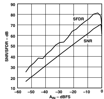
TPC 27. SNR/SFDR vs. A IN (Input Amplitude) (f IN = 5.0 MHz, Input Span = 2 V p-p, V CM = 2.5 V)
