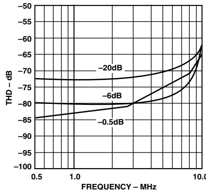
TPC 23. THD vs. Input Frequency (Input Span = 2.0 V p-p, V CM = 2.5 V)
