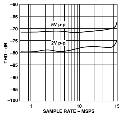
TPC 26. THD vs. Clock Frequency (A IN = -0.5 dB, f IN = 1.0 MHz, V CM = 2.5 V)
