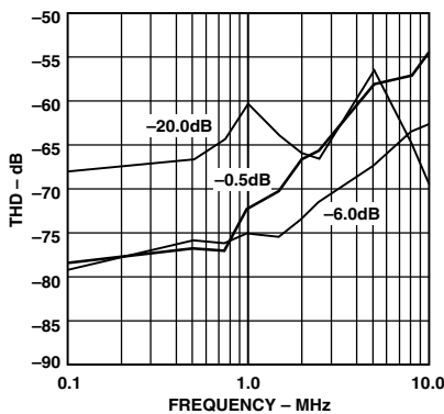
TPC 25. THD vs. Input Frequency (Input Span = 5.0 V p-p, V CM = 2.5 V)
