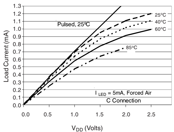
Figure 4. Typical On-Characteristic C Connection
