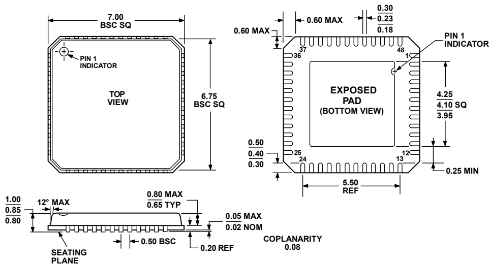
COMPLIANT TO JEDEC STANDARDS MO-220-VKGD-2 Figure 71. 48-Lead Frame Chip Scale Package [LFSCP_VQ] 7 mm × 7 mm Body, Very Thin Quad (CP-48-3) Dimensions shown in millimeters
