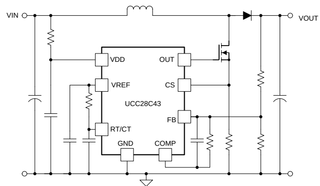
Simplified Schematic
