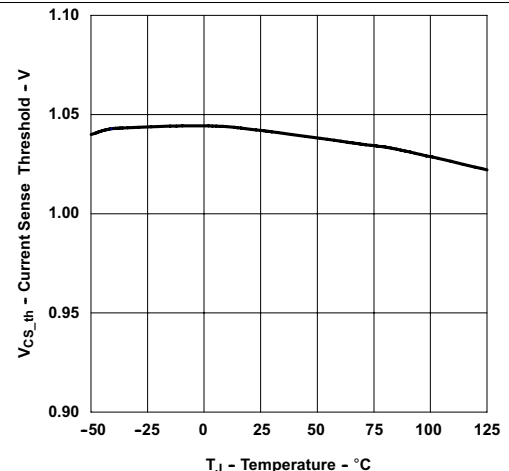
Figure 18. Current Sense Threshold Voltage vs Temperature
