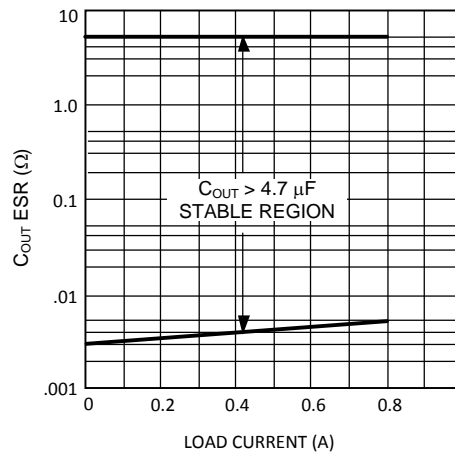
Figure 19. Minimum ESR vs Output Load Current
