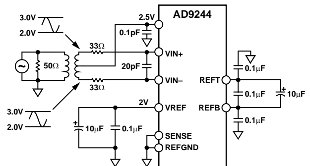
Figure 42. 2 V p-p Differential Input, Common-Mode Voltage = 2.5 V
