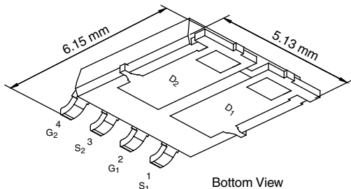
PowerPAK® SO-8L Dual
