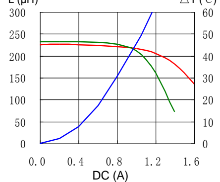
21. CDRH124NP-221MC
