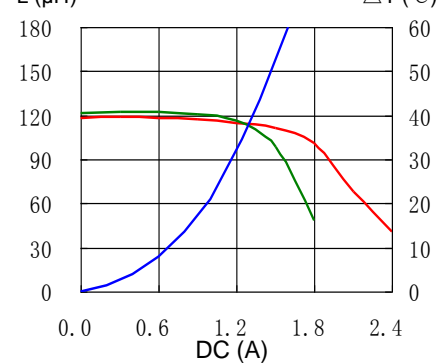
21. CDRH124NP-221MC
