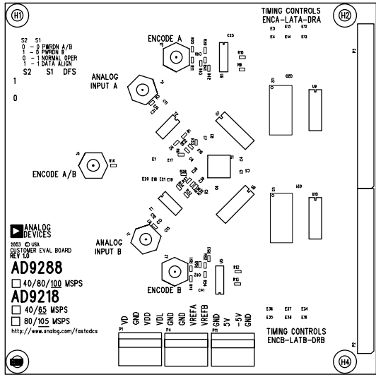
Figure 28. Top Silkscreen
