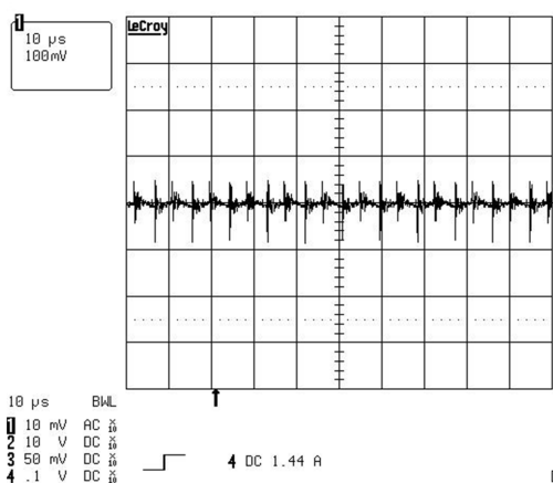
Figure 41. Output Voltage Ripple at Full Load (100 mV/div)
