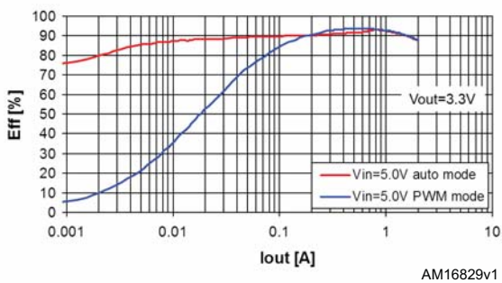
Figure 9. Efficiency vs. output current (PWM/auto mode V_{IN} = 5.0\text{ V} )
