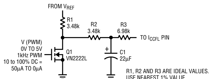
LT1184/LT1184F I CCFL PWM Programming with V REF
