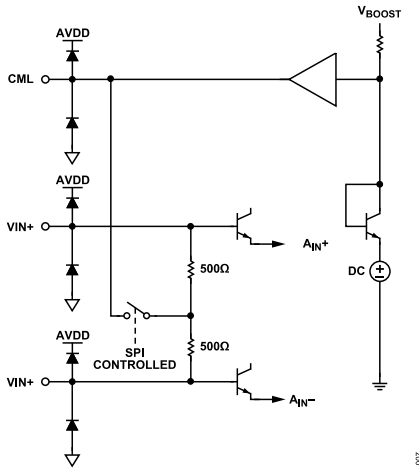
Figure 34. Analog Input DC Equivalent Circuit ( V_{CML} \sim 1.7\text{ V} )
