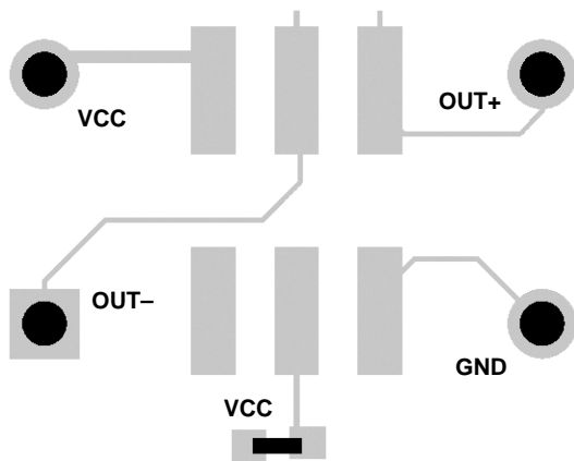
Figure 38. XTAL Footprint
