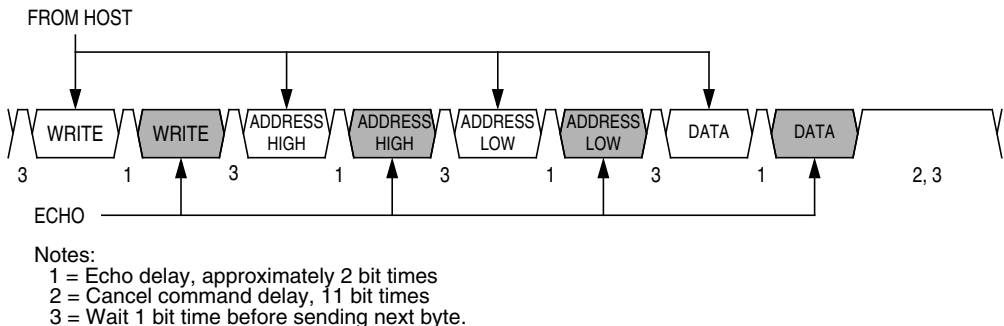
Figure 8-6. Write Transaction
