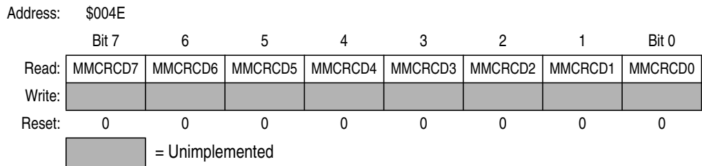
Figure 14-10. MMIIC CRC Data Register (MMCRCDR)
