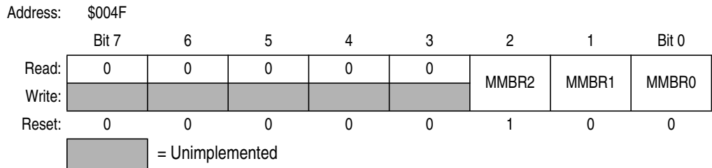
Figure 14-11. MMIIC Frequency Divider Register (MMFDR)
