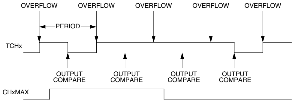
Figure 9-11. CHxMAX Latency
