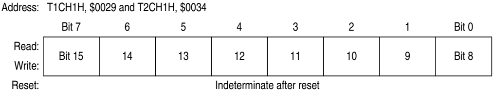
Figure 9-14. TIM Channel 1 Register High (TCH1H)
