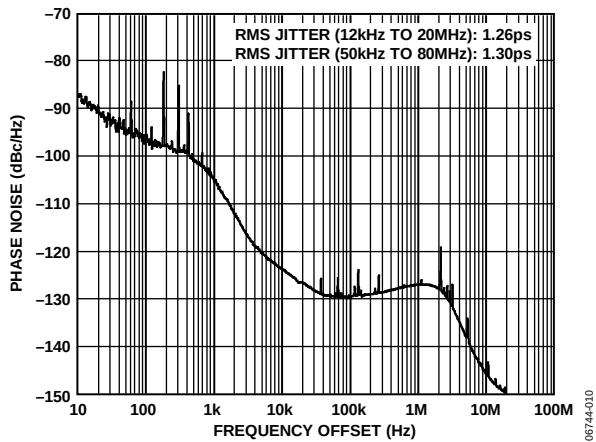
Figure 10. Additive Phase Noise at HSTL Output Driver, SYSCLK = 1 \text{ GHz} ( SYSCLK PLL Enabled and Driven by a 25 MHz Fox Crystal Oscillator), f_{REF} = 19.44 \text{ MHz} , f_{OUT} = 155.52 \text{ MHz} , DPLL Loop BW = 1 kHz
