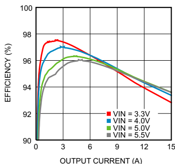
Efficiency at 2.5 V, 500 kHz
