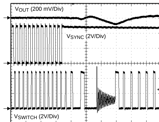
Figure 16. SYNC Signal Removed, 4 \mu\text{s/Div}
