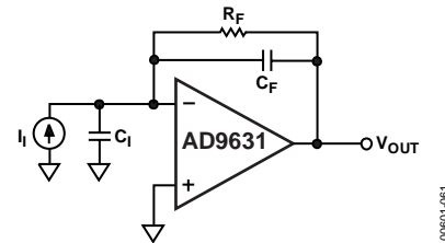
Figure 61. Transimpedance Configuration
