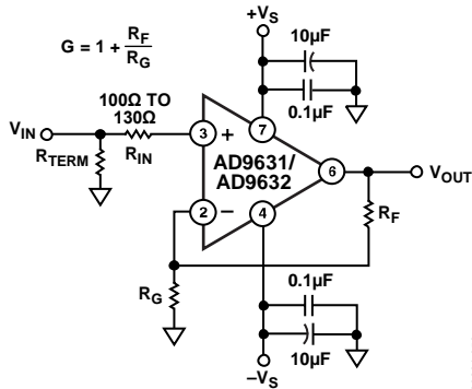
Figure 59. Noninverting Operation
