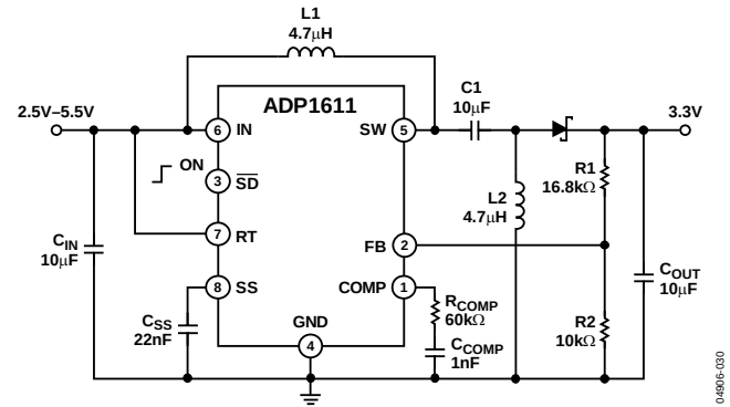
Figure 30. 3.3 V DC-to-DC Converter
