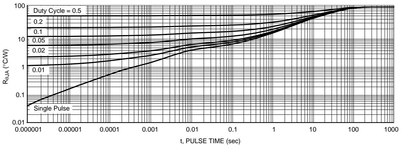
Figure 5. Thermal Response
