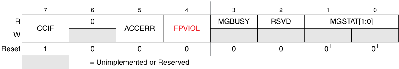
Figure 24-11. Flash Status Register (FSTAT)
