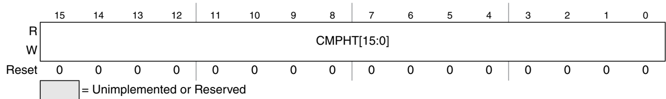
Figure 15-13. ATD Compare Higher Than Register (ATDCMPHT)
