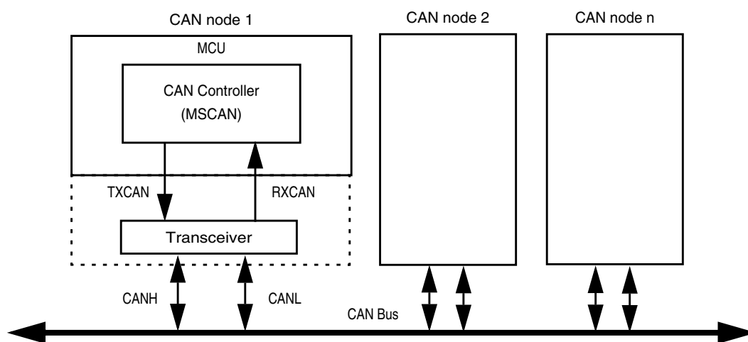
Figure 18-2. CAN System
