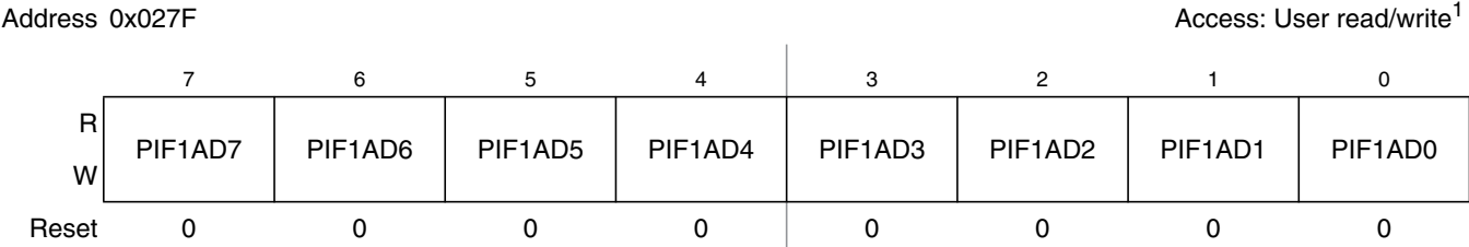
Figure 2-63. Port AD Interrupt Flag Register (PIF1AD)
