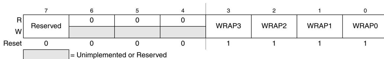
Figure 15-3. ATD Control Register 0 (ATDCTL0)
