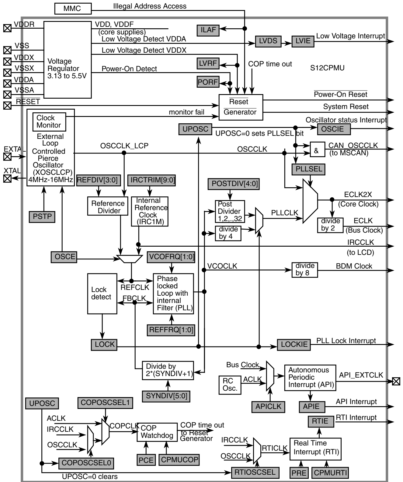
Figure 10-1. Block diagram of S12CPMU
