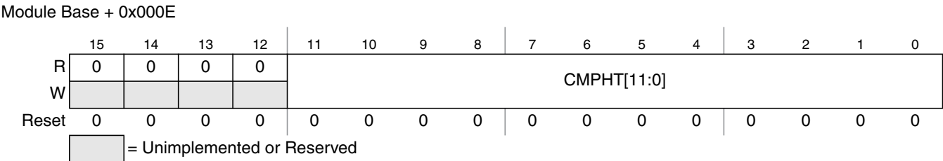
Figure 14-13. ATD Compare Higher Than Register (ATDCMPHT)
