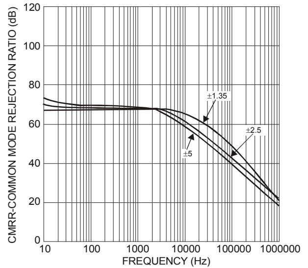
Figure 6 Common Mode Rejection Ratio vs. Frequency
