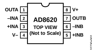
Figure 2. 8-Lead SOIC_N
