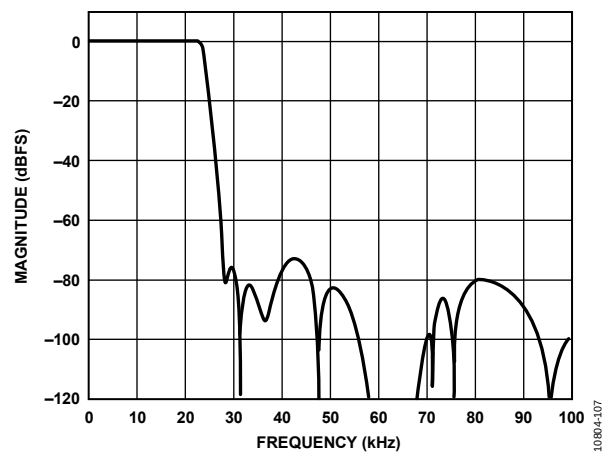
Figure 74. Total Interpolation Response, f_s = 192 kHz
