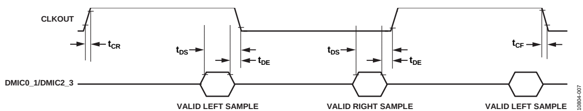
Figure 7. Digital Microphone Timing
