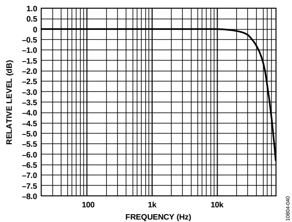
Figure 41. Relative Level vs. Frequency, f_s = 192 kHz, Signal Path = DAC_SDATA to ASRC to LOU TLx
