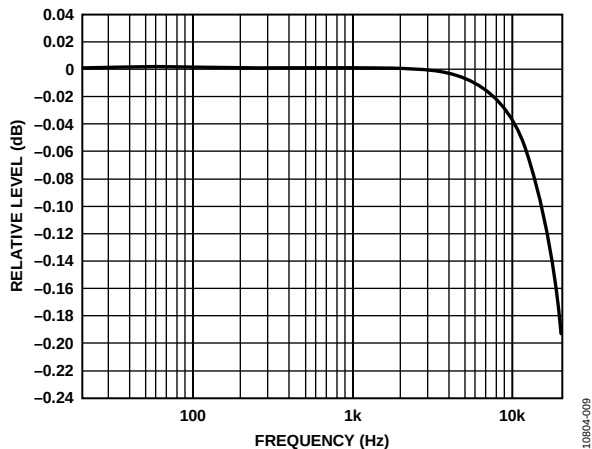
Figure 10. Relative Level vs. Frequency, f_s = 48 kHz, Signal Path = AIN0 to DSP (Without Processing) to LOU TLx
