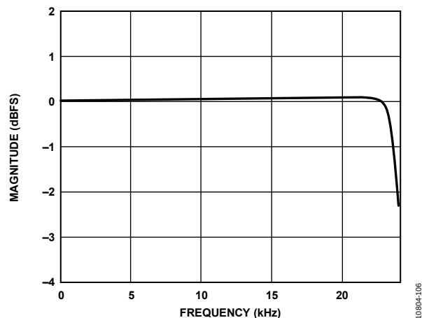
Figure 73. Interpolation Pass-Band Response, f_s = 192 kHz
