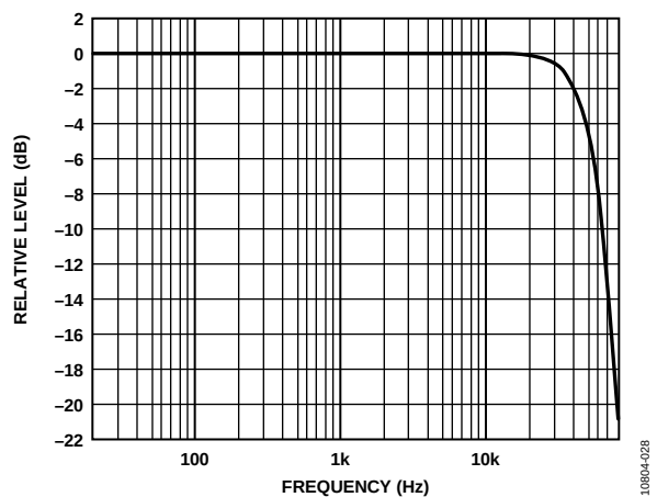
Figure 29. Relative Level vs. Frequency, f_s = 192 kHz, Signal Path = AIN0 to ASRC to ADC_SDAT00
